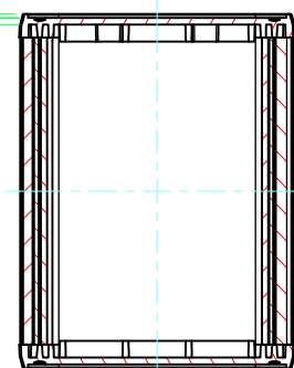
C-C (1:1.5)
