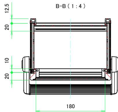
B-B (1:4)
