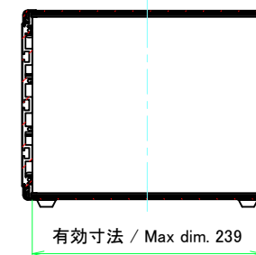
C-C (1:5)
