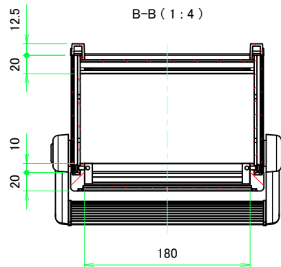
B-B (1:4)
