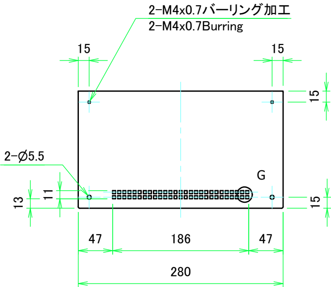
C view
