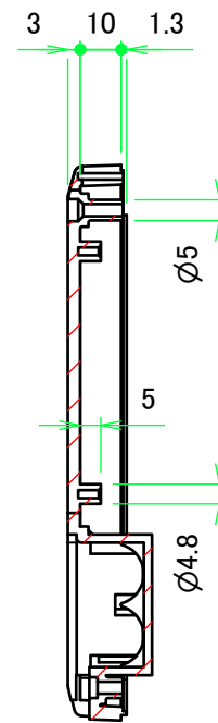
E-E (1:2)
