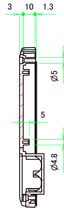
E-E (1:2)
