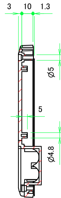
E-E (1:2)
