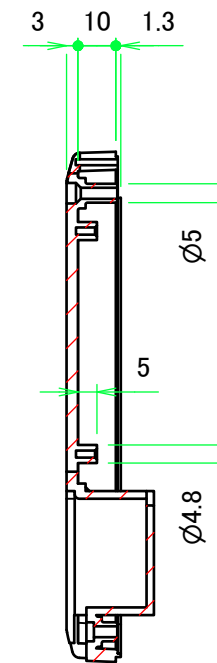
E-E (1:2)
