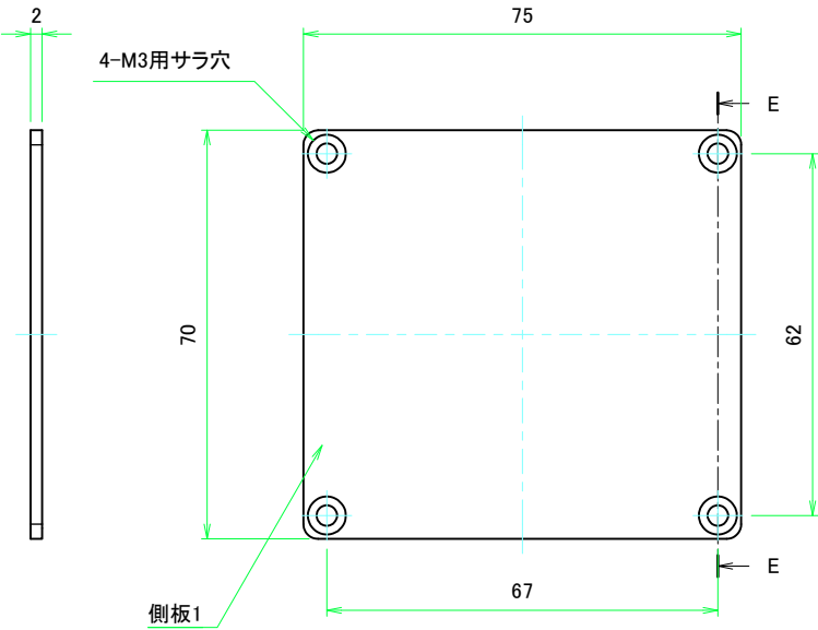
E-E (1:1)
