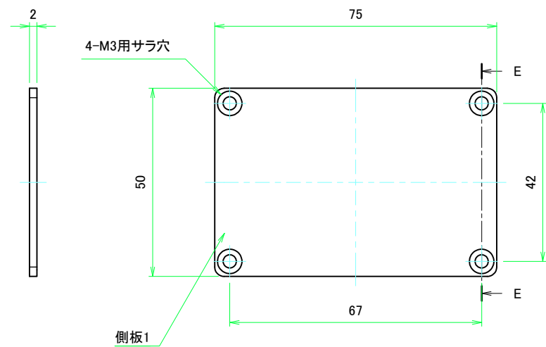
E-E (1:1)
