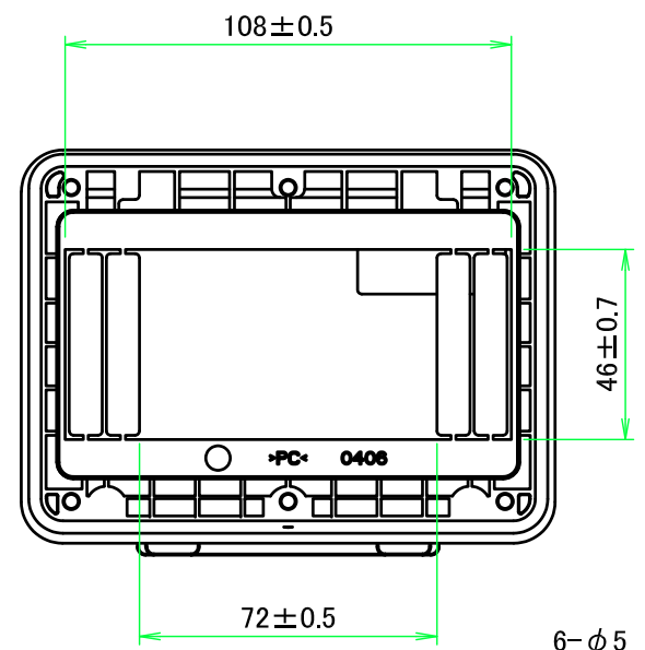
取付穴加工図 / Hole layout for mounting
