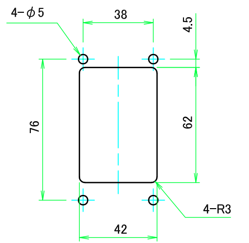
取付穴加工図 / Hole layout for mounting
