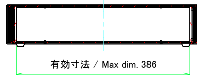
B-B (1:6)
