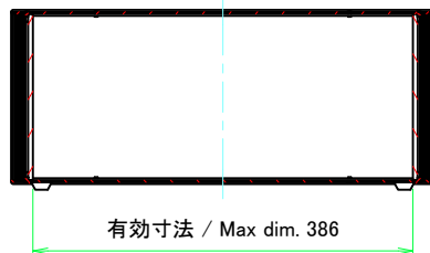
B-B (1:6)
