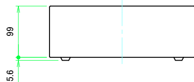
B-B (1:5)
