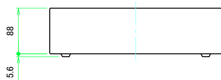
B-B (1:5)
