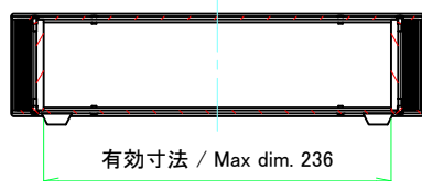
B-B (1:4)
