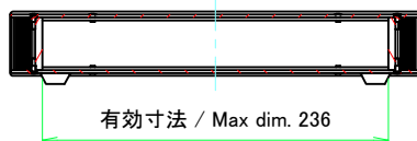
B-B (1:4)
