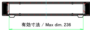
B-B (1:4)
