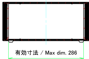
B-B (1:6)
