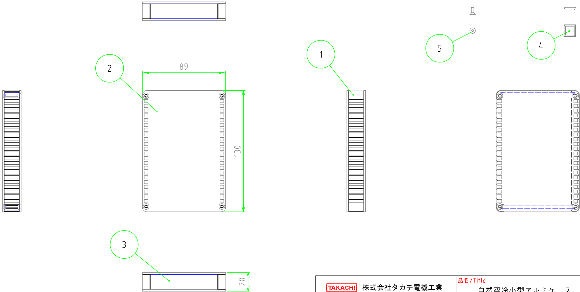
ゴム足 / Self-adhesive rubber feet
