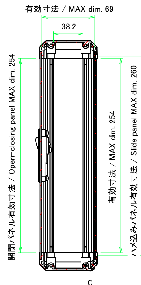
B-B (1:3)
