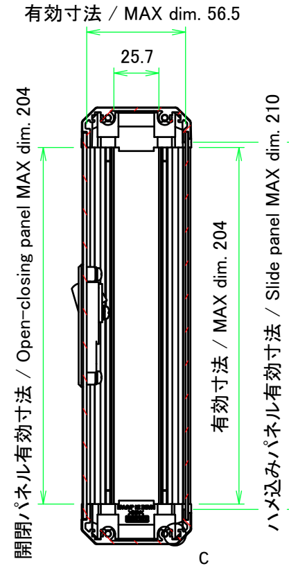
B-B (1:3)
