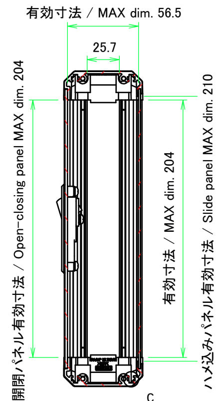
B-B (1:3)
