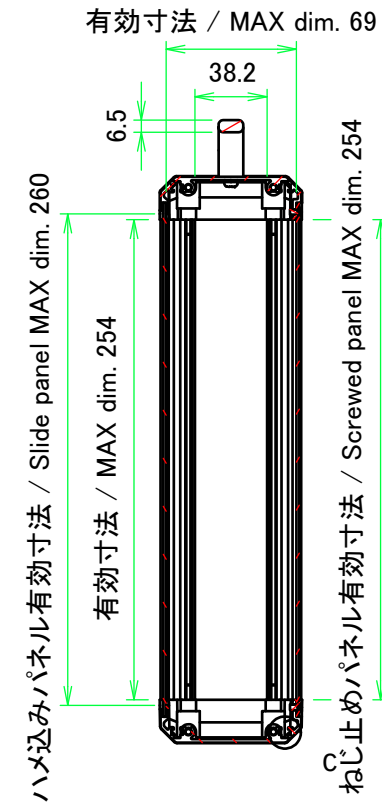
B-B (1:4)
