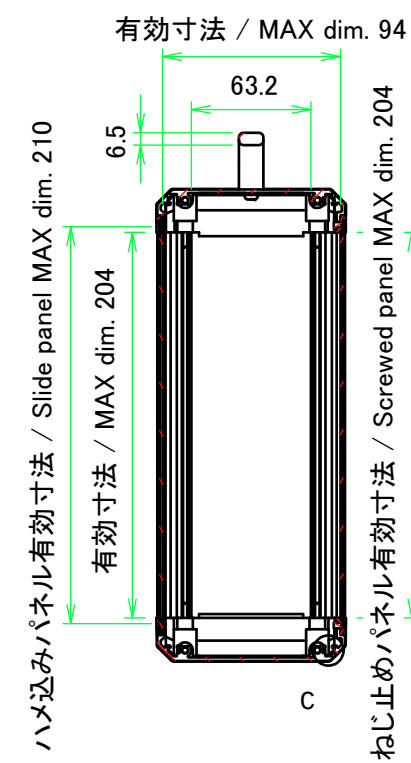
B-B (1:4)
