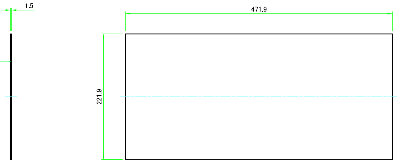
パネル裏面/Panel Backside
