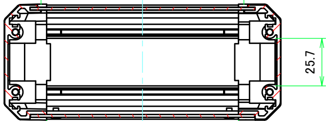
ねじ止めパネル有効寸法 / Screwed panel Max dim. 104
