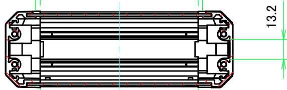
ねじ止めパネル有効寸法 / Screwed panel Max dim. 104
