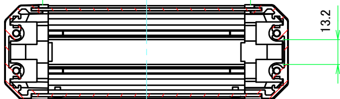
ねじ止めパネル有効寸法 / Screwed panel Max dim. 104
