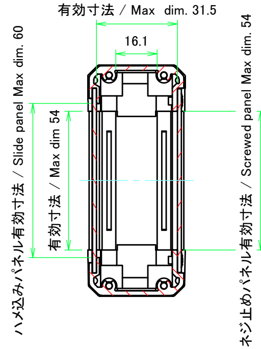
B-B (1:1.5)
