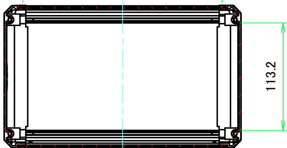
ねじ止めパネル有効寸法 / Screwed panel Max dim. 204
