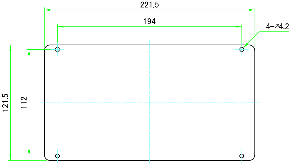
パネル裏面/Panel Backside
