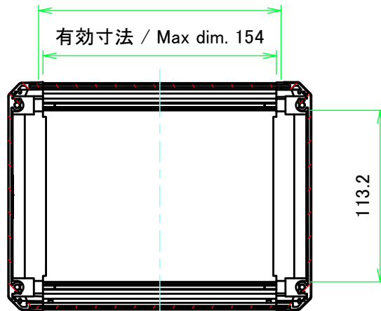
ねじ止めパネル有効寸法 / Screwed panel Max dim. 154
