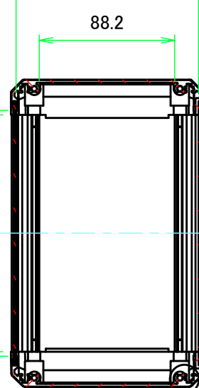
ねじ止めパネル有効寸法 / Screwed panel Max dim. 154
