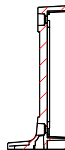
B-B (1:3)
