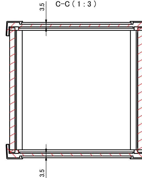
C-C (1:3)
