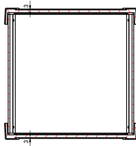
C-C (1:2.5)
