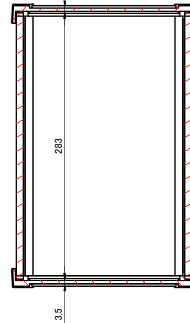
C-C (1:4)
