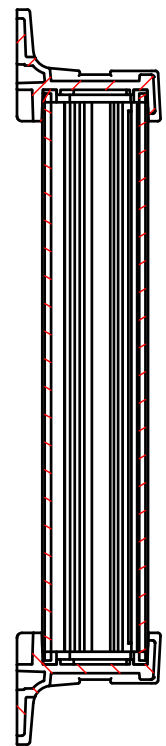
B-B (1:3)
