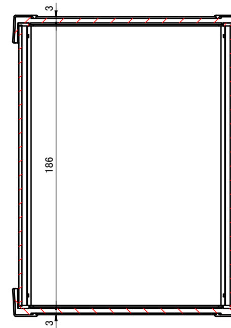
C-C (1:2.5)
