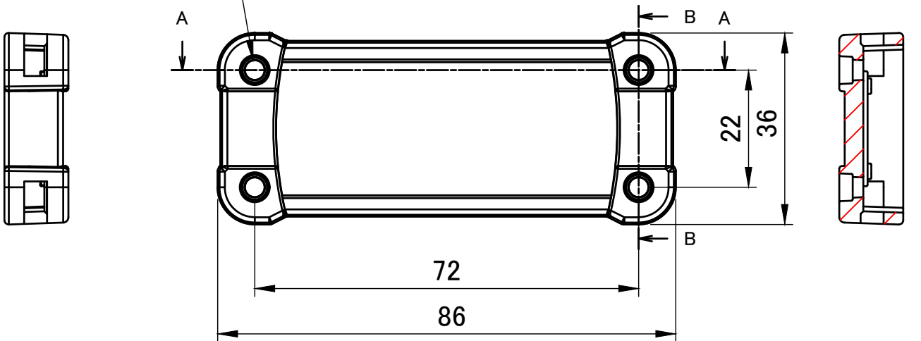
B-B (1:1)
