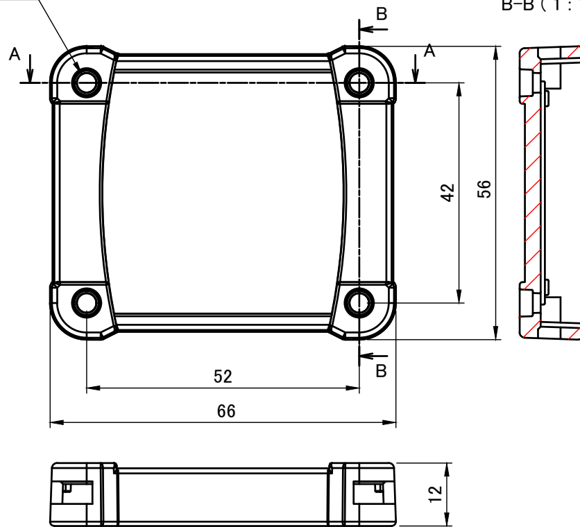
B-B (1:1)
