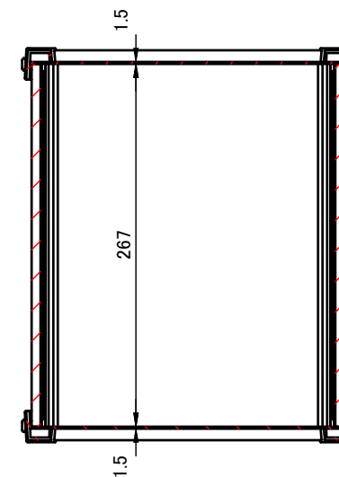
C-C (1:5)
