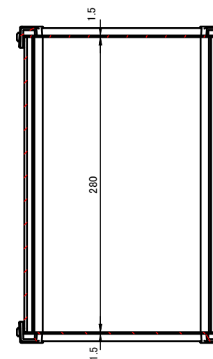
C-C (1:5)
