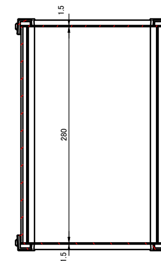
C-C (1:5)
