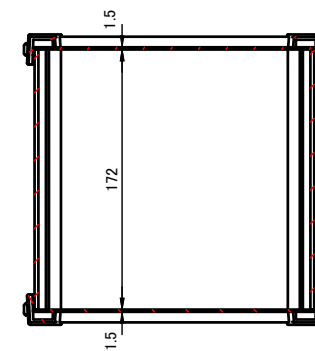
C-C (1:5)
