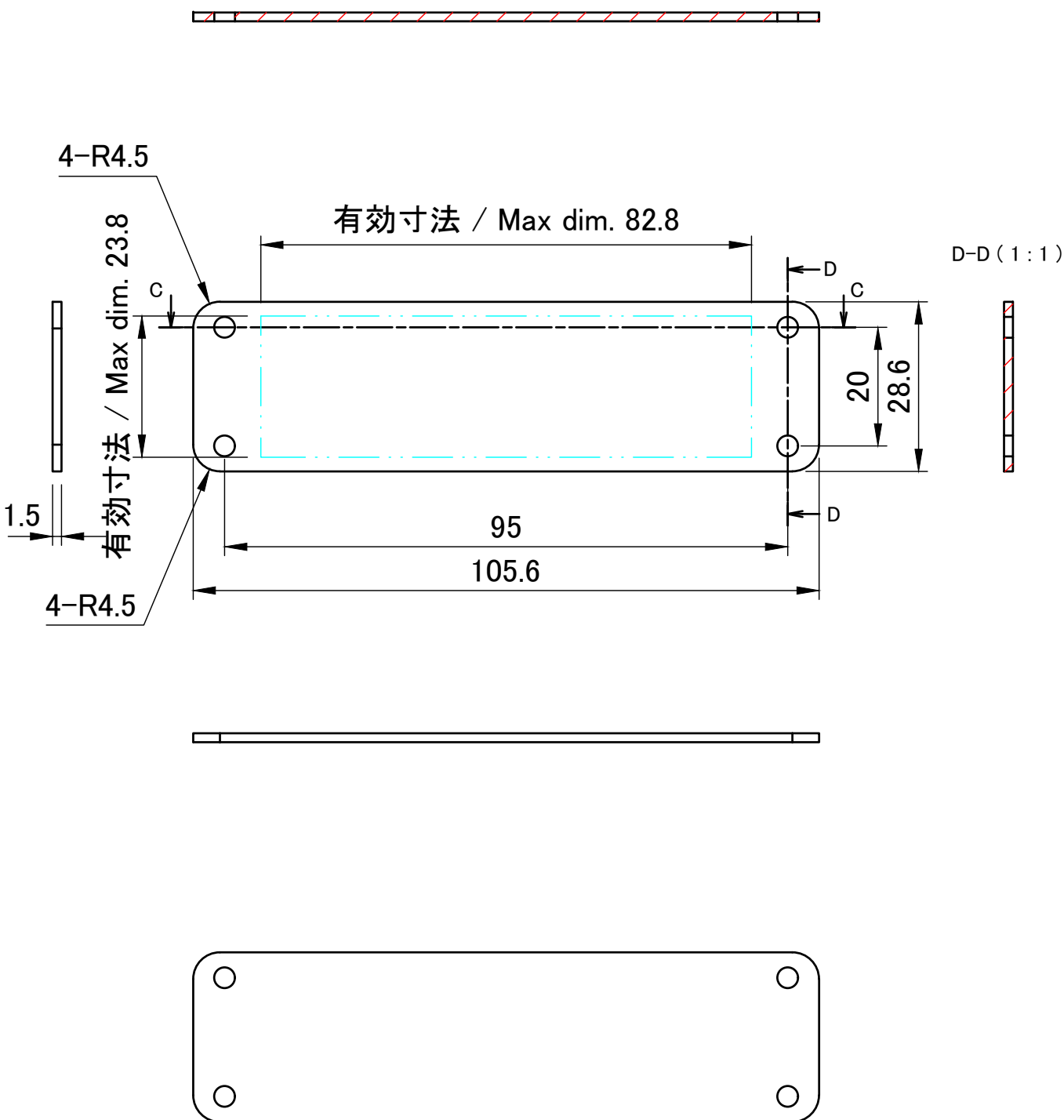
C-C (1:1)
