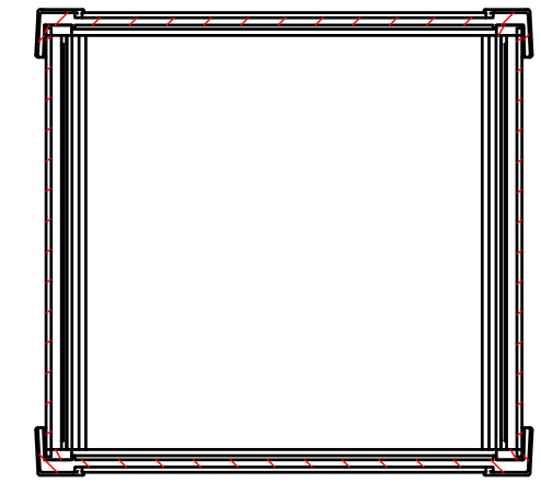
C-C (1:4)
